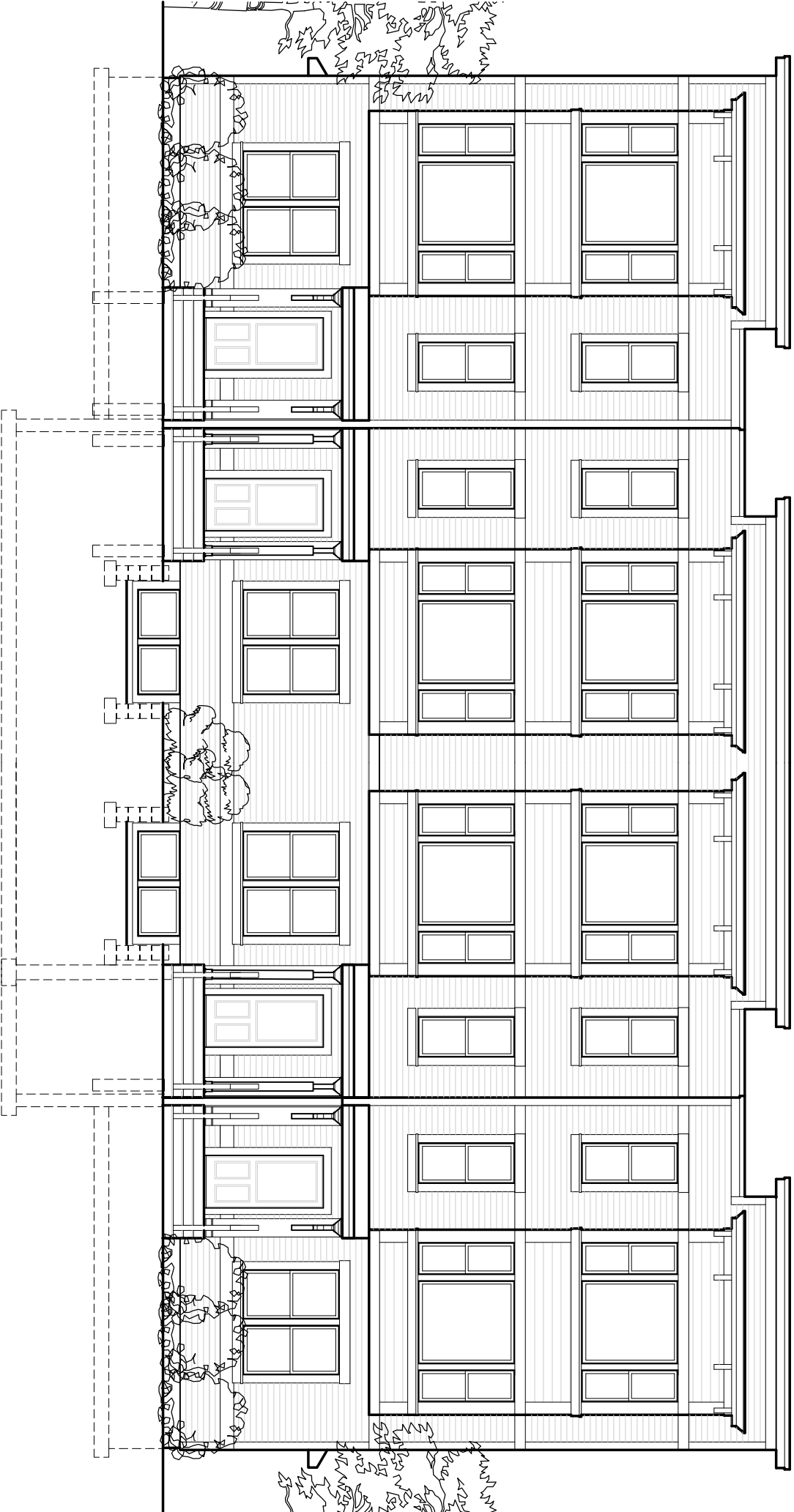
FRONT ELEVATION UNITS 5,6,7,8,9,10
