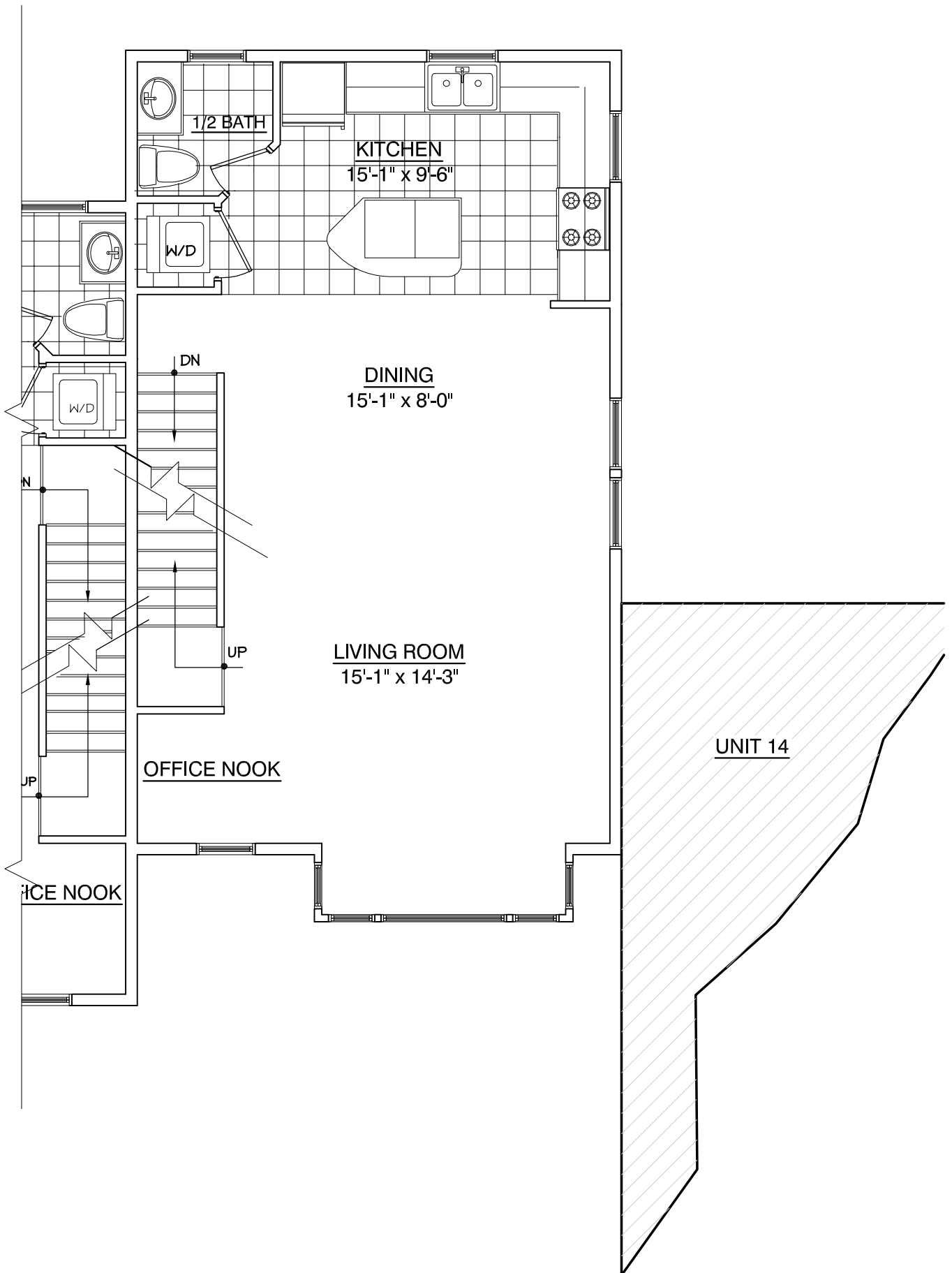
SECOND FLOOR PLAN UNIT 12
