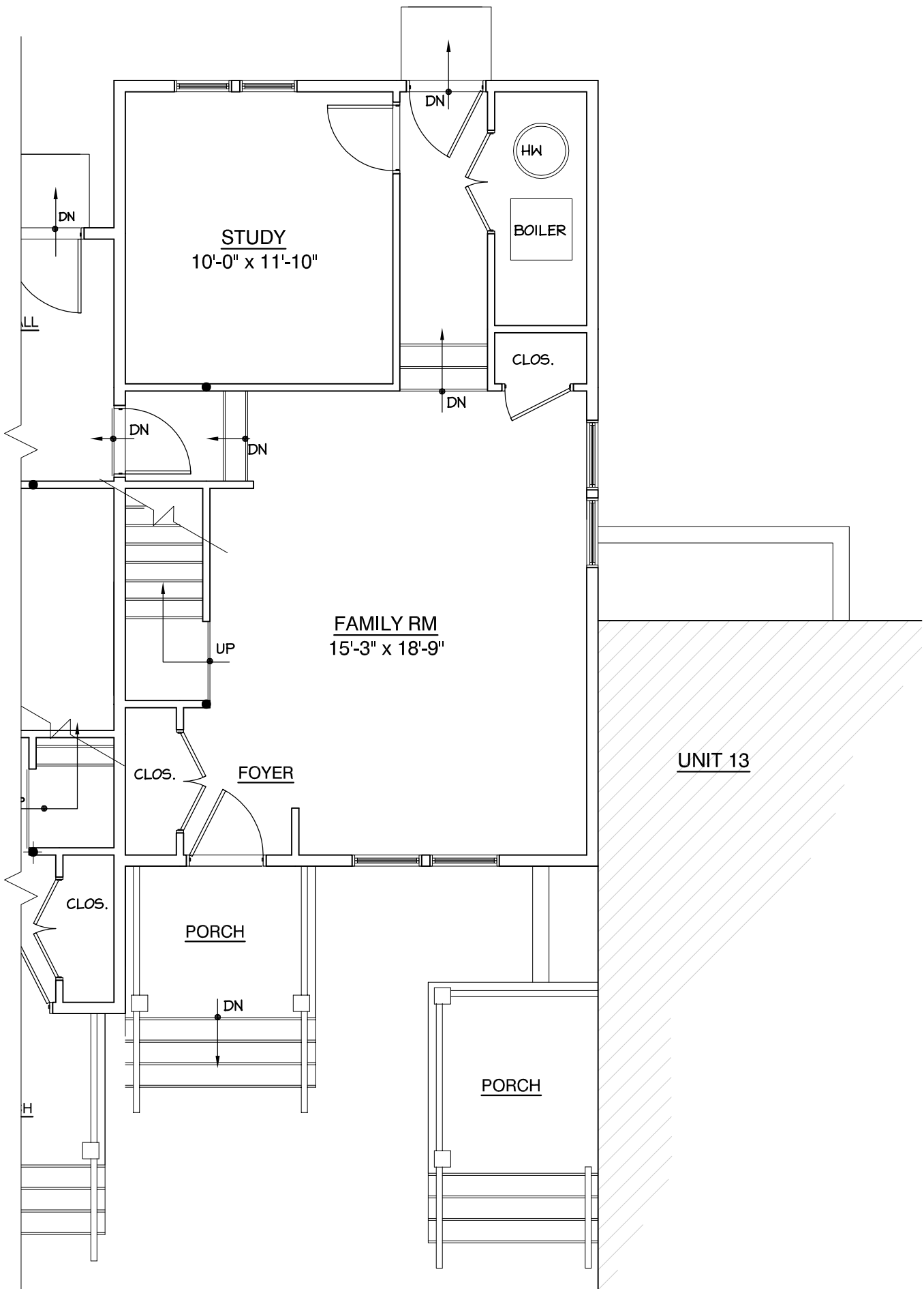
FIRST FLOOR PLAN UNIT 12
